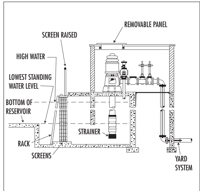
VERTICAL SHAFT TURBINE-TYPE FIRE PUMP INSTALLATION IN WET PIT
