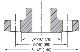
1-1/4" (32) ANSI 250 lb. (113 kg) 4-Bolt Flange
